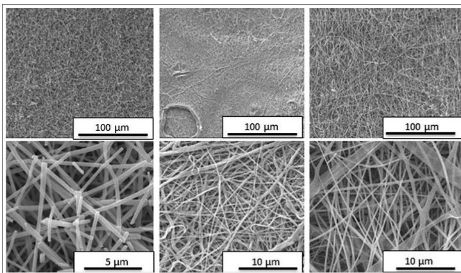
Fig. 1. SEM images of titanium dioxide fiber samples templated with PVP. (Left column: ET1, middle column: ET2, right column: ET3).
