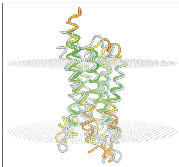
G-protein coupled receptor: in grey the crystallographically solved structure and – in color – a model. The color gradient corresponds to a predicted quality score. The cell membrane is represented with white balls. (Copyright University of Basel)
