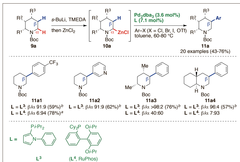
Scheme 5. β-Arylation of Boc-piperidines. a Yield of the isolated mixture of α and β isomers.
