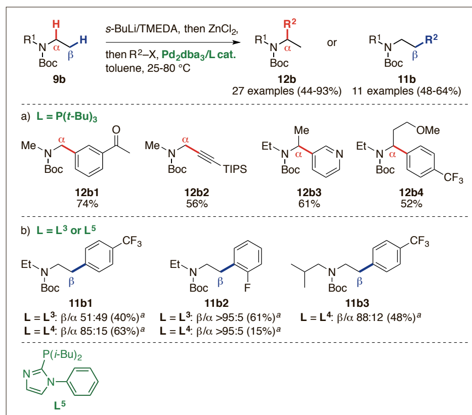
Scheme 6. Ligand-controlled α- and β-arylation of acyclic Boc-amines. a Yield of the isolated β isomer.
