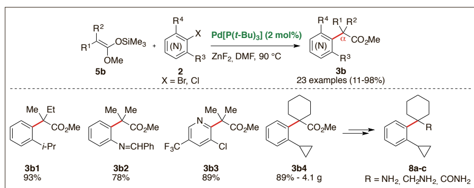
Scheme 4. \alpha -Arylation of hindered silyl ketene acetals and (hetero)aryl halides.
