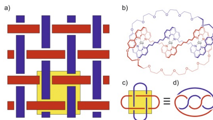
Fig. 1. a) Sketch of a biaxial woven fabric. b) Trinuclear Cu(II) complex resulting in a doubly interlocked [2]-catenane sketched in d) upon removal of the copper ions. c) Alternative representation of the doubly interlocked [2]-catenane as Solomon knot. The analogy of the Solomon knot with the unit cell of the fabric is highlighted by a yellow square.
