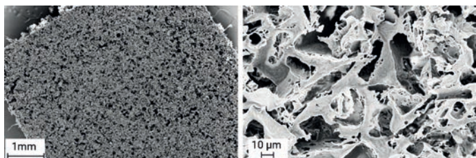
Fig. 1. SEM micrographs of open porous biopolymer foams with interconnecting voids obtained by salt leaching with 80–100 μm NaCl crystals suspended into a matrix of poly(3-hydroxybutyrate-co-3-hydroxyvalerate) copolymer.
